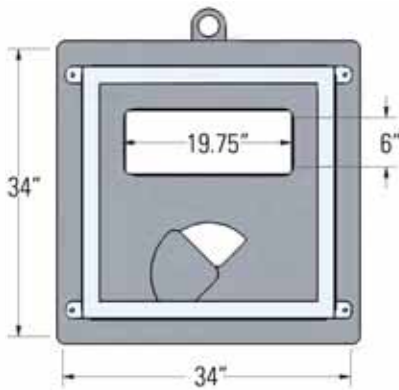
Outside Measurements
