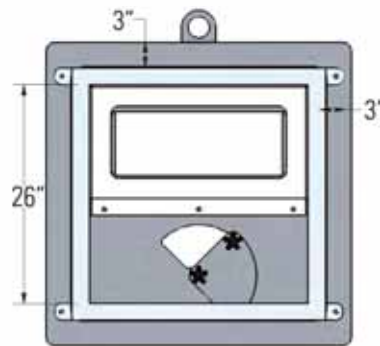
Inside Measurements
